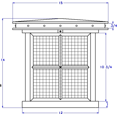
# 80590-ind-ir-pil-ba Iron Industrial Pilaster Lantern Bar-stock iron transitional lighting Shown with Text Bronze Finish & Clear Glass - 14" height x 15" w -
